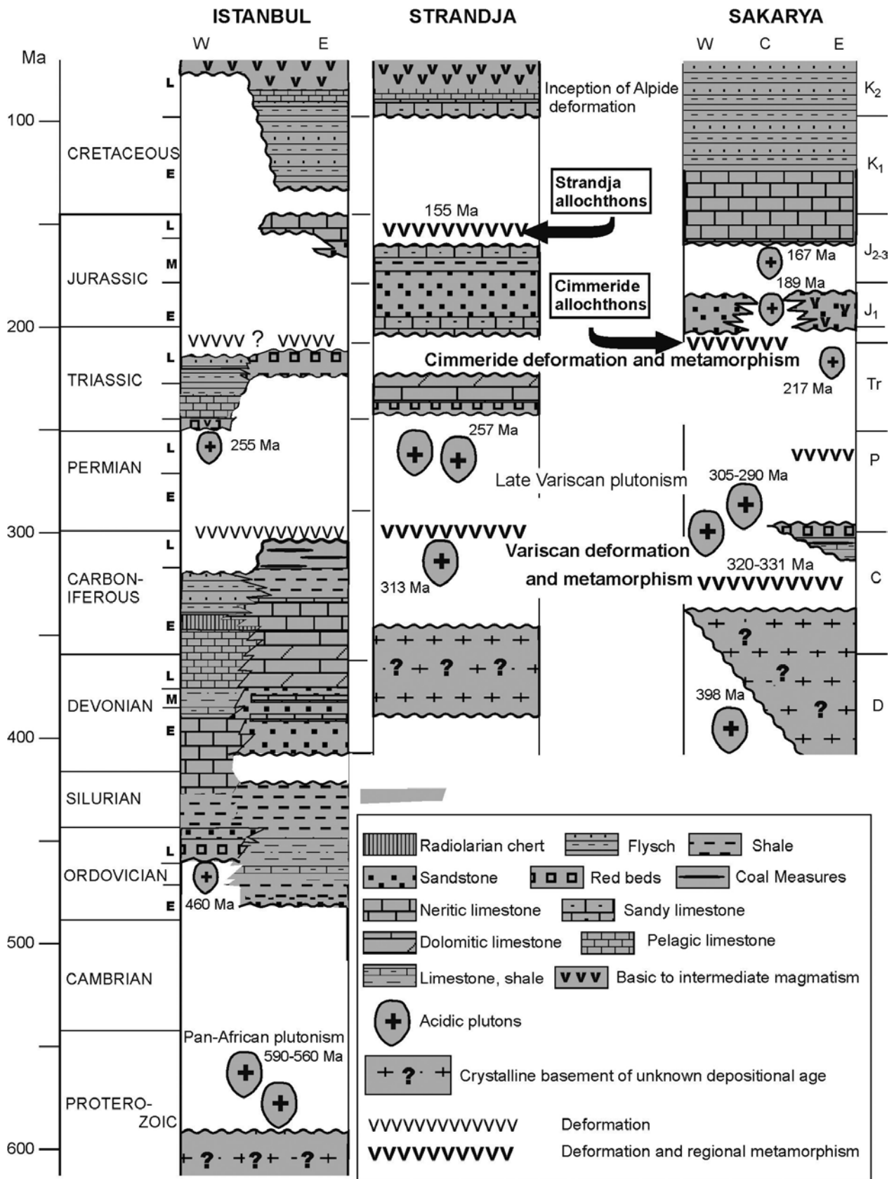
Fig. 5: Synthetic stratigraphic sections of the Istanbul, Strandja and Sakarya Zone terranes (Okay et al. 2008).
